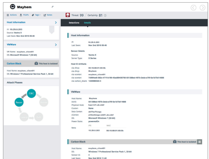
The Vectra UI shows that Carbon Black isolated a compromised host that was initially detected and assigned threat and certainty scores by Vectra
